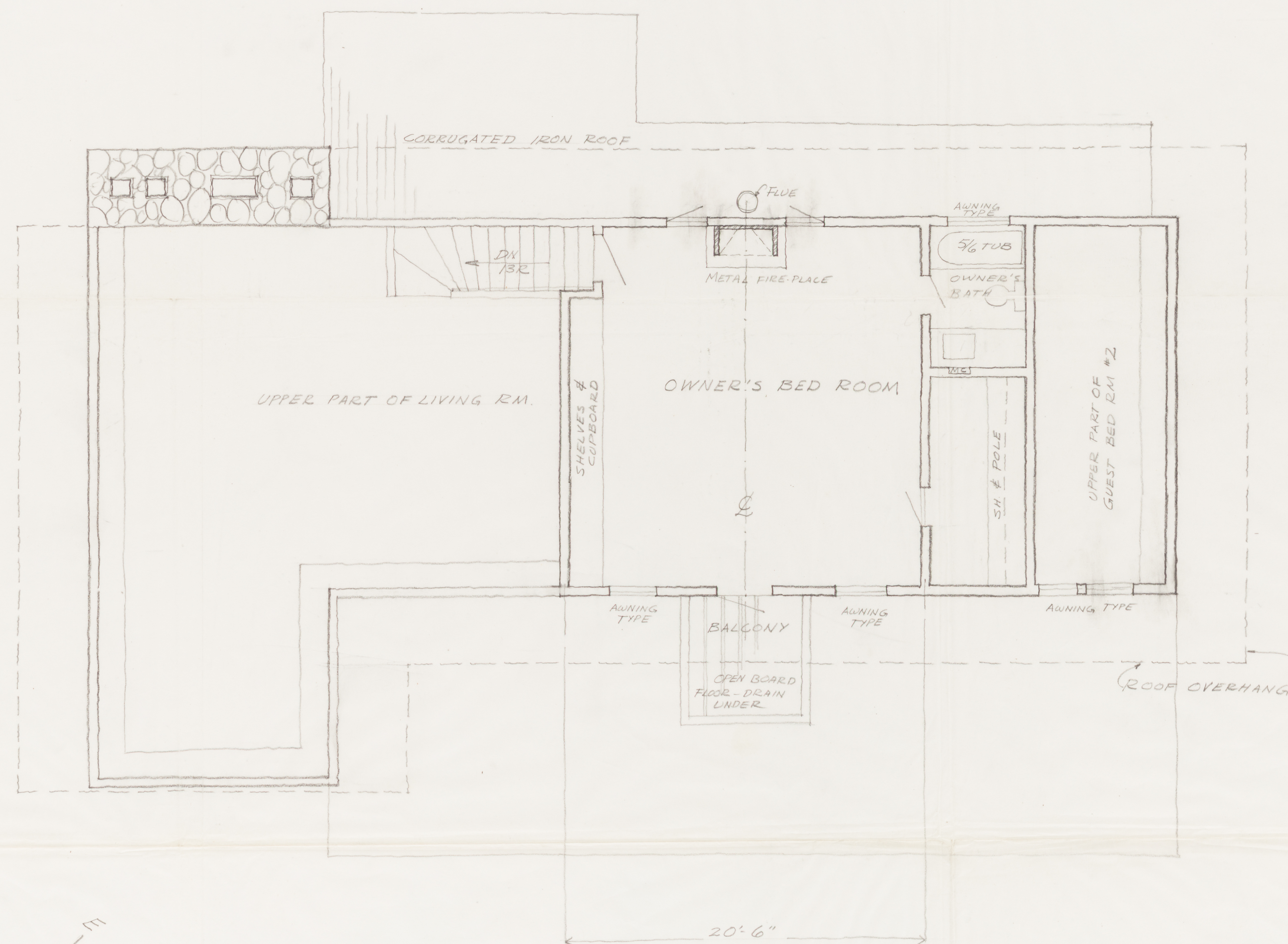
SECOND FLOOR PLAN \frac{1}{4}" = 1'-0" SCALE
